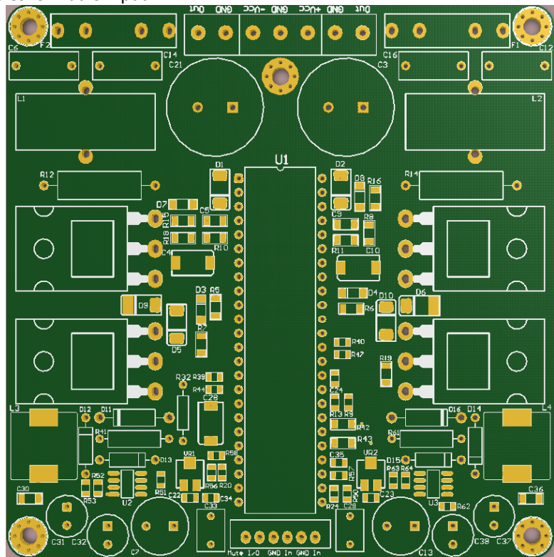
Figure 4: TA3020 Audio Amplifier Module Board layout overview and connections
